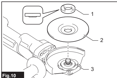
Fig. 10 ► 1. Lock nut 2. Depressed center wheel 3. Inner flange
