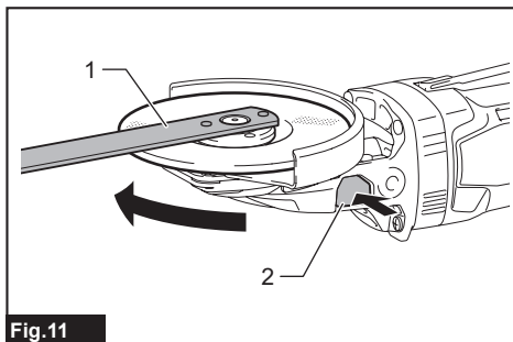
Fig. 11 ► 1. Lock nut wrench 2. Shaft lock
