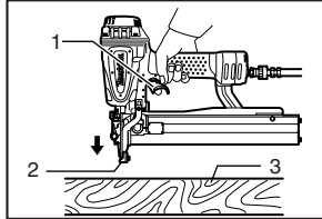
1. Trigger 2. Contact element 3. Workpiece
