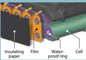
Waterproof Triple-layer Structure prevents cell failure due to water and dust.
