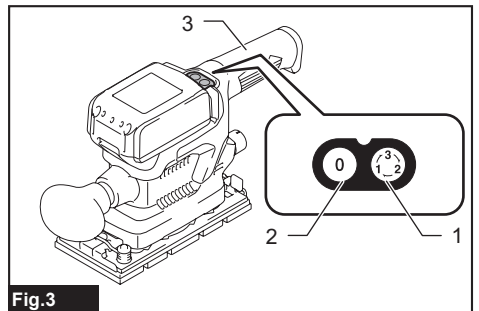
► 1. Power/speed select button 2. Stop button 3. Main handle
