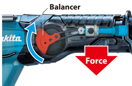
Smooth cutting with vertical crank system
