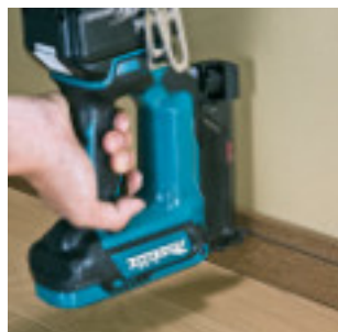
Nails can be fired in the groove of baseboard.
