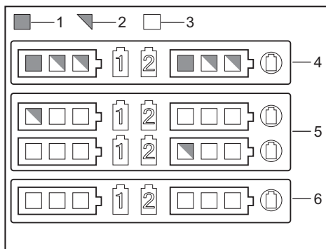
► 1. Lighting 2. Blinking 3. Turned off 4. Overheat protection 5. Overdischarge protection 6. Overload protection
